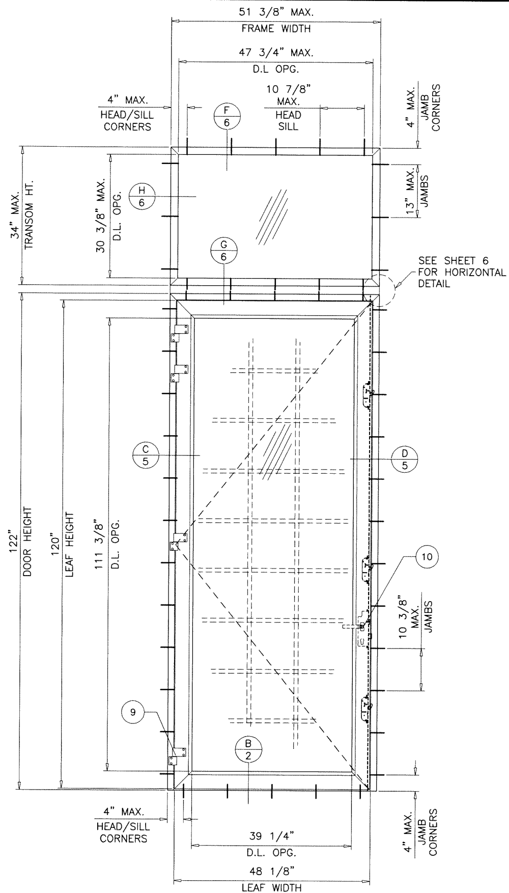
TYPICAL ELEVATION ( O/X )
